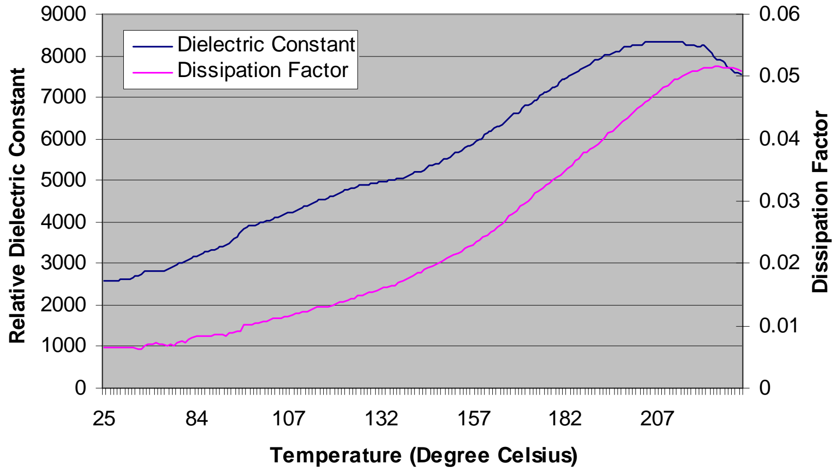
DL-48 Temperature Dependence of Dielectric Properties
