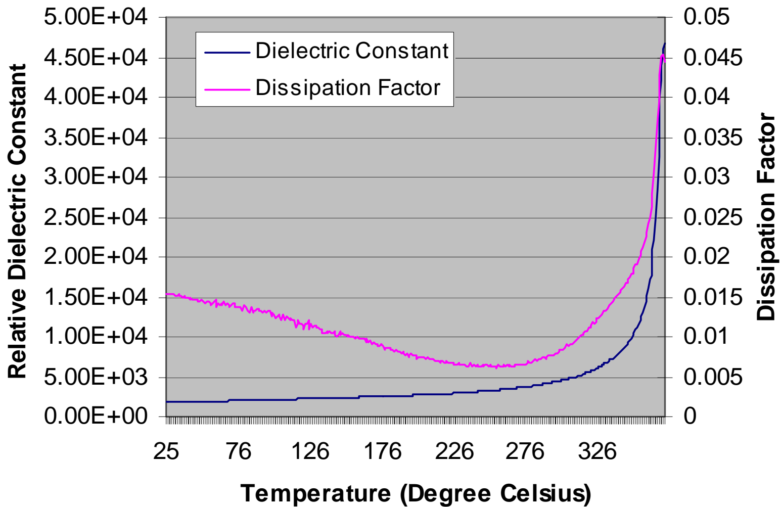
DL-50 Temperature Dependence of Dielectric Properties
