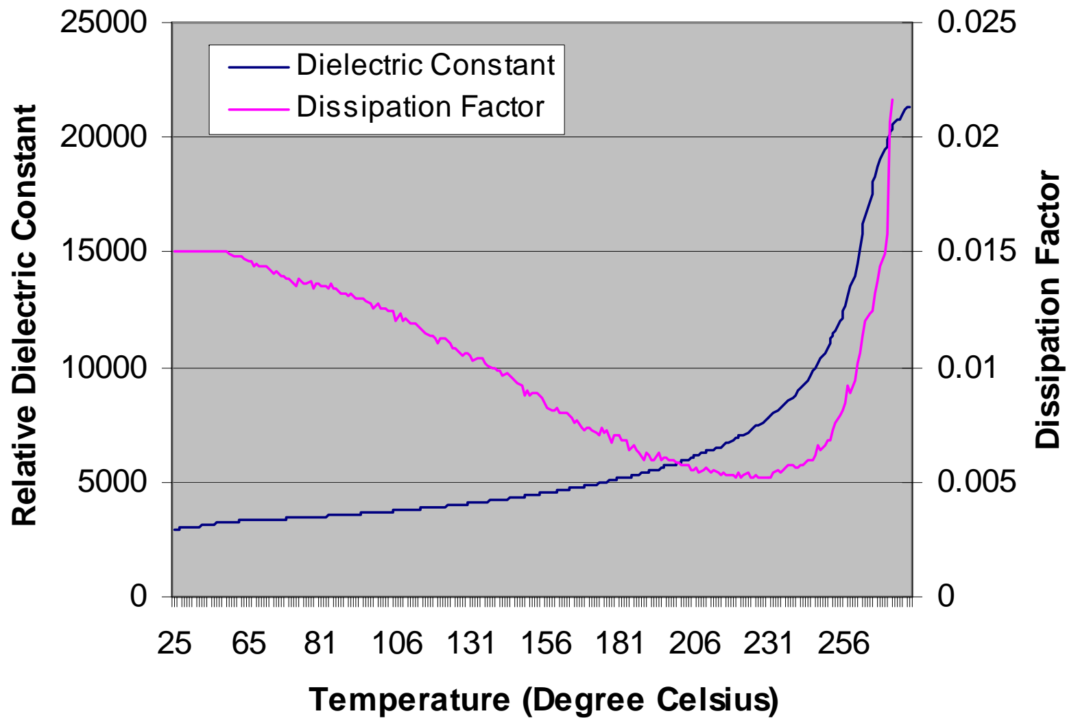
DL-52 Temperature Dependence of Dielectric Properties
