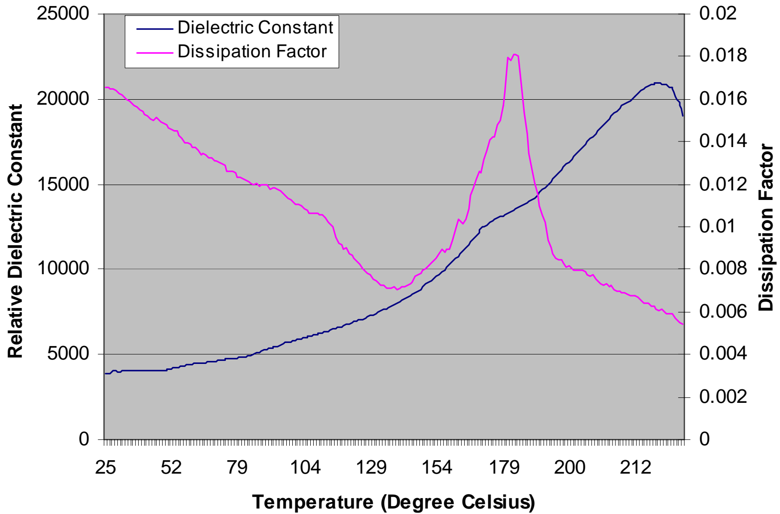
DL-53HD Temperature Dependence of Dielectric Properties
