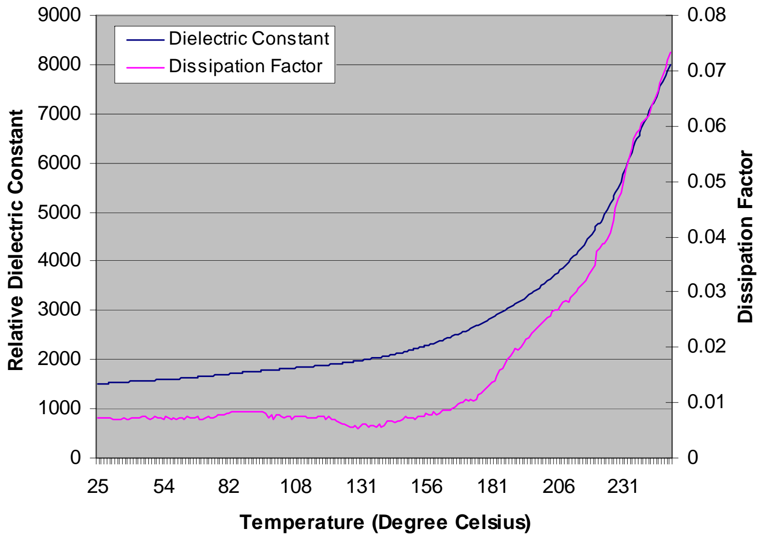
DL-46 Temperature Dependence of Dielectric Properties
