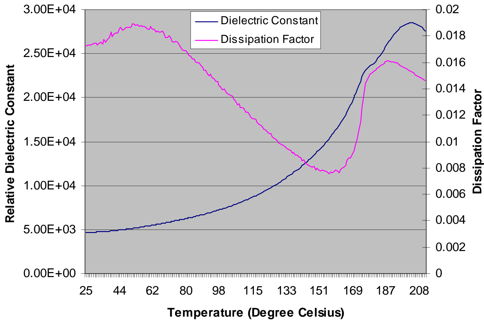
DL-54HD Temperature Dependence of Dielectric Properties
